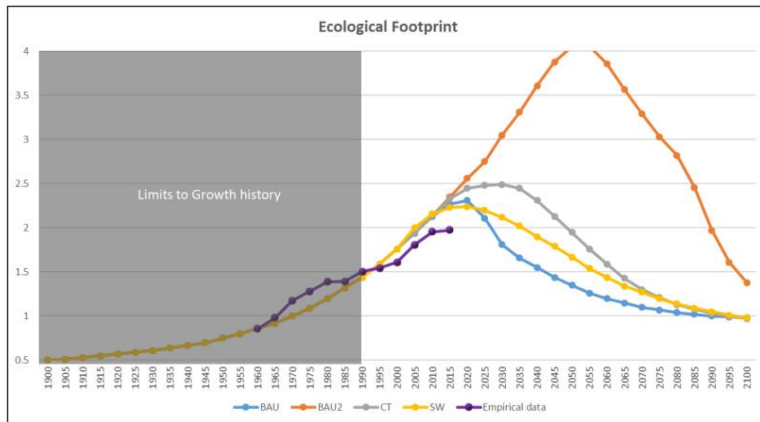
Figure S1-10. Scenarios and empirical data for the human ecological footprint.
